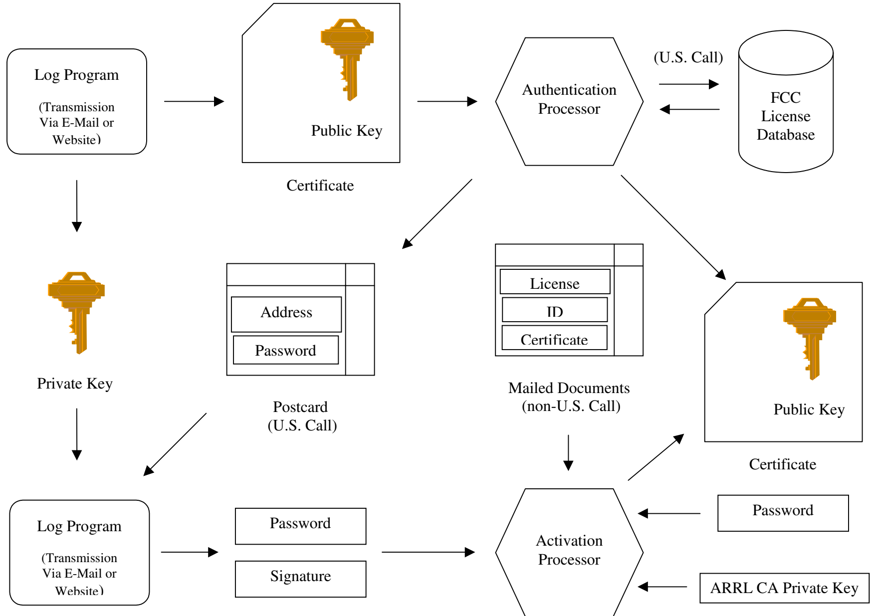
Fig. 2.1 - Authentication Protocol
